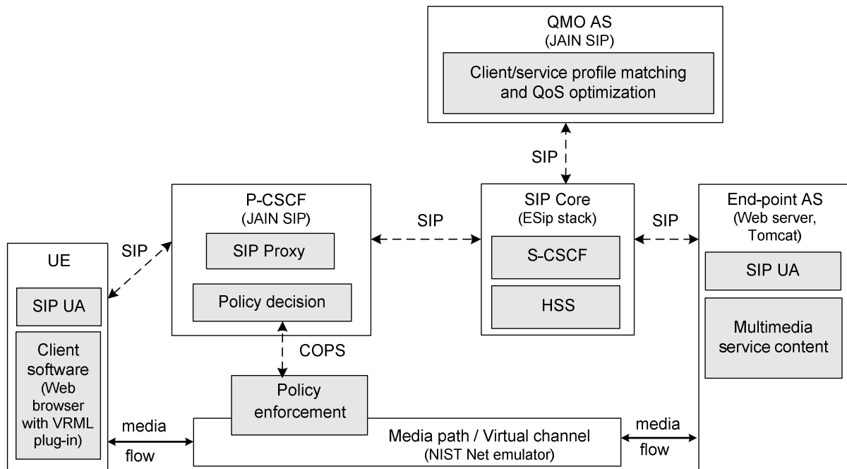
Figure 6 – Logical view of the testbed.
