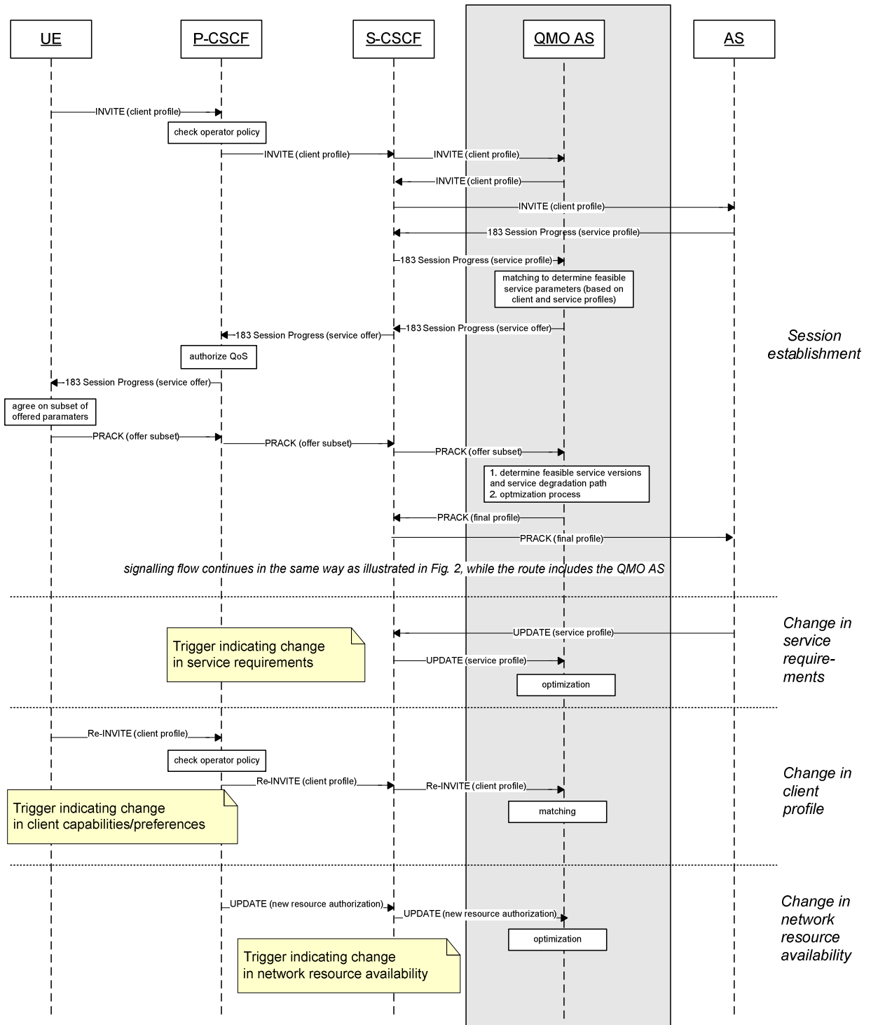
Figure 5 – SIP signaling in the case study
